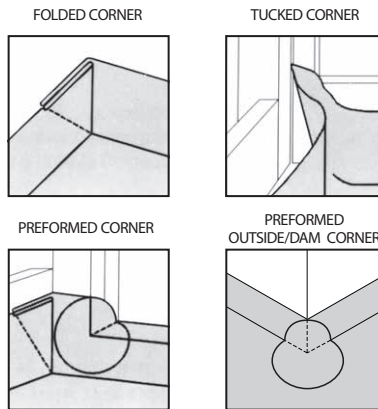
FIGURE 4. CORNERS
