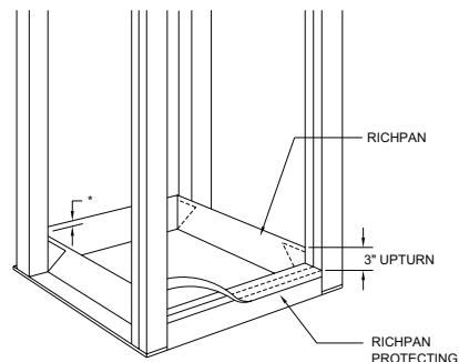
FIGURE 2. SHOWER PAN
